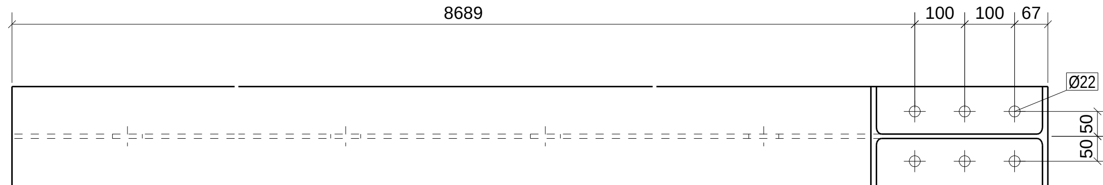
TOP VIEW
